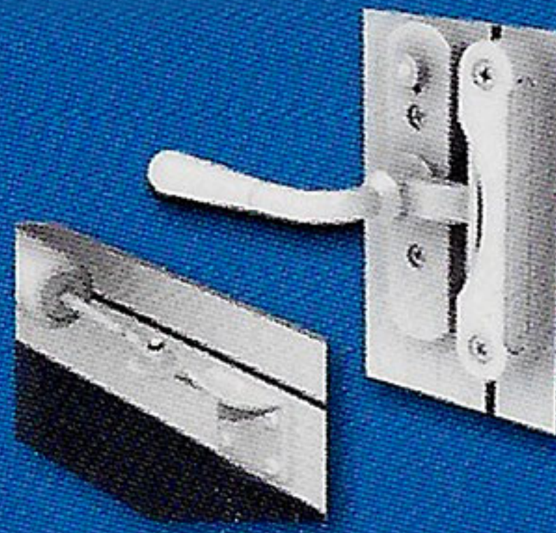
Albright In-Swing Handle and Closer Tube Bracket
